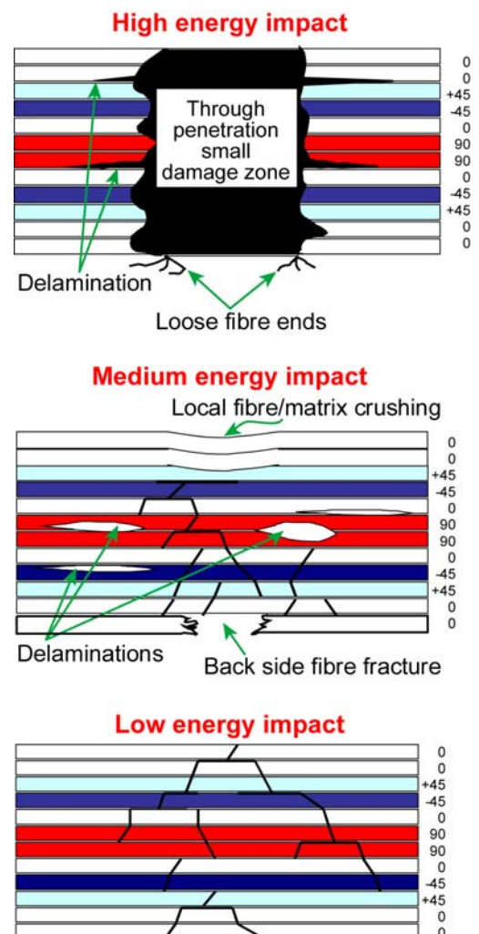
Figure 1: Levels of damage Photo courtesy Abaris Training [6]
