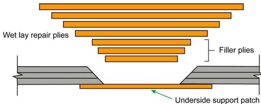
Figure 2: Laminated Patch Repair
