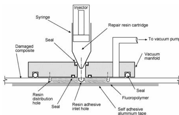
Figure 6 - Resin Infusion or Injection Repair
