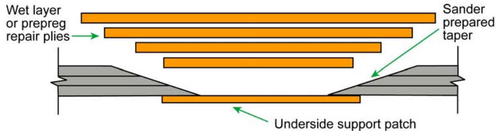
Figure 3b: Tapered Scarf Repair
