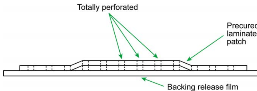
Figure 4 - Adhesive Bonded Doubler
