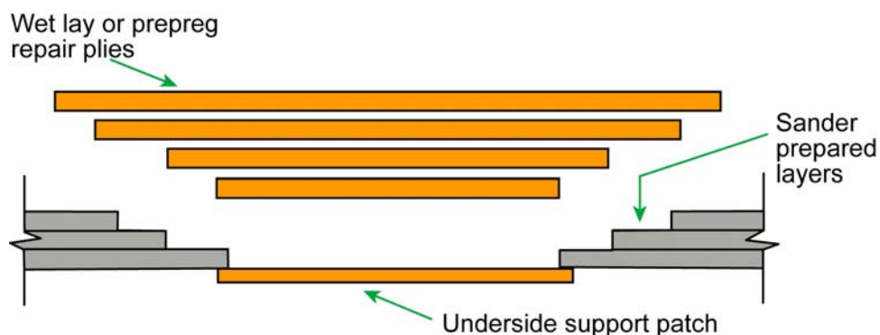
Figure 3a: Stepped Scarf Repair
